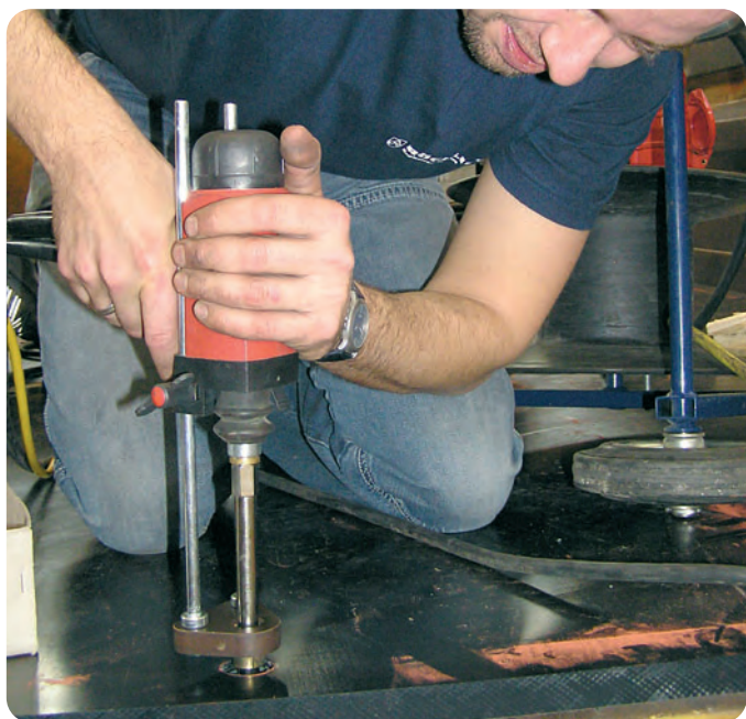
Fixing system Stud weld
